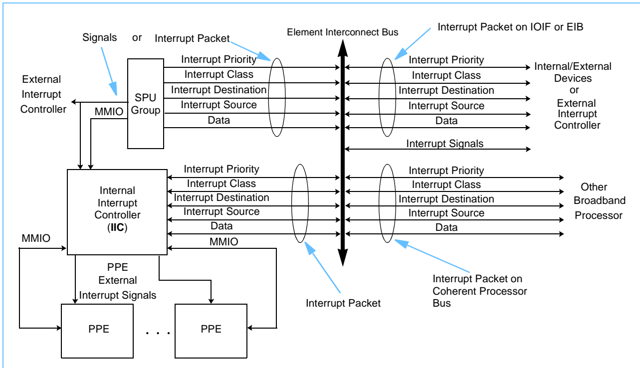
Figure 21-1. Interrupt Presentation
